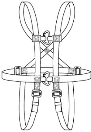
Construction of Rappelling System ( not include D-SHAPE carabiner )
